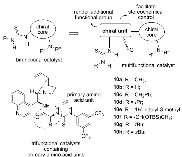
Scheme 2. Novel trifunctional catalysts containing an amino acid unit. FG = functional group, TBS = tert -butyldimethylsilyl.
