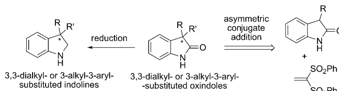
Scheme 1. Construction of 3,3-dialkyl-substituted or 3-alkyl-3-aryl-disubstituted oxindoles and indolines. R = aryl or alkyl, R' = alkyl.
