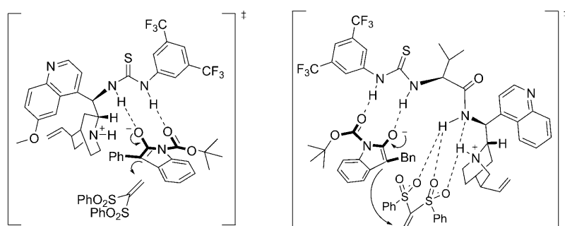
Scheme 4. Plausible reaction mechanisms.
