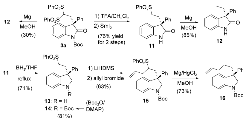
Scheme 3. Synthesis of 3-alkyl-3-aryl-disubstituted oxindole and indoline. DMAP=4-dimethylaminopyridine, HMDS = 1,1,1,3,3,3-hexamethyldisilazane, TFA=trifluoroacetic acid, THF=tetrahydrofuran.
